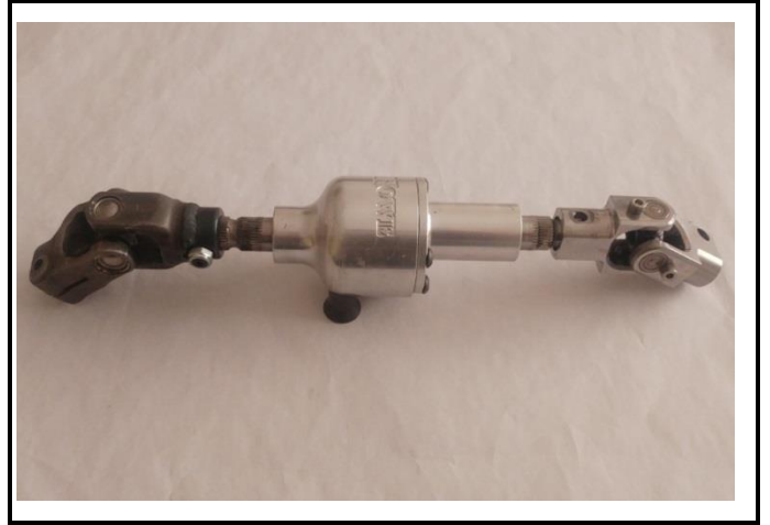
PHOTO 4: 804-c,d Steering multiplier, disassembled.
