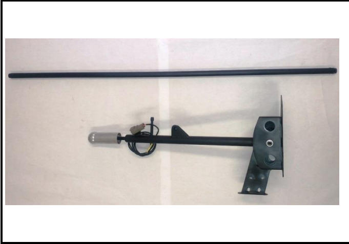
PHOTO 3: 603 Gear lever type 2 with shorter ratio.
