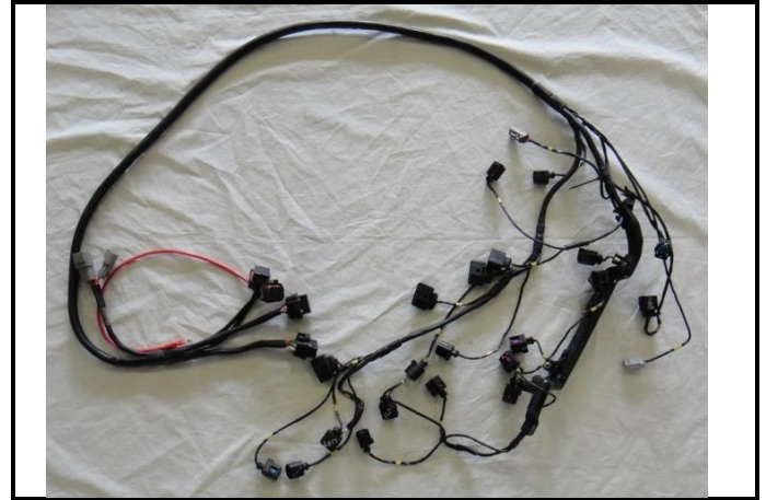
PHOTO 10: 324c9, Engine electrical harness.
