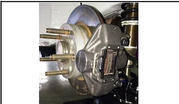
K3-1) Rear brake assembly – zoom on caliper and support
