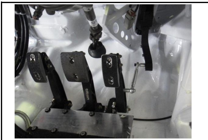
PHOTO 5: 803 b, Brake pedal box, type 2, mounted.
