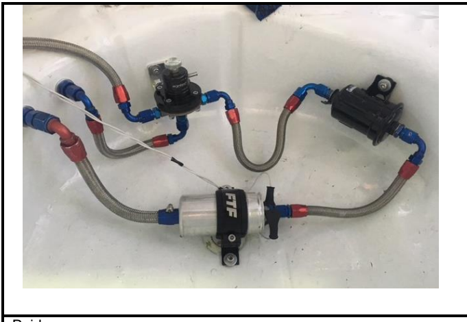
D1-4) Fuel pumps in their location
