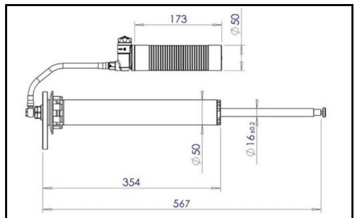
AA2) Front Damper Drawing
