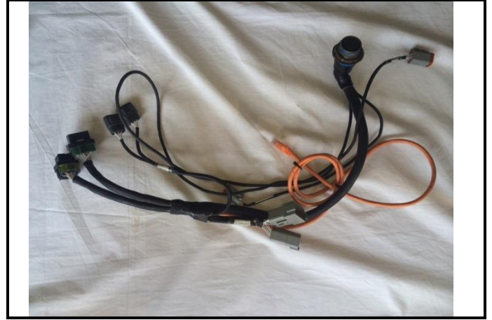
4) ECU harness.
