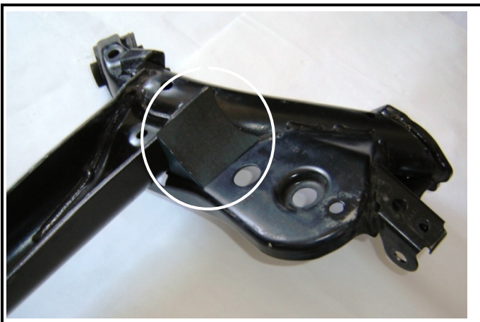
1) Reinforced rear axle. Type 4. Top.
