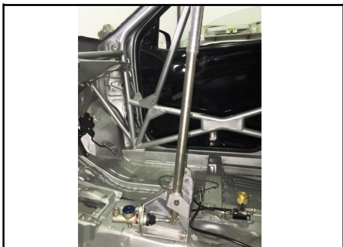
Photo 3: J8-1): Handbrake type 3 mounted.
