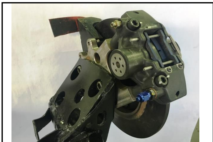
Photo 5. K3-1): Rear brake caliper, type 2, mounted.
